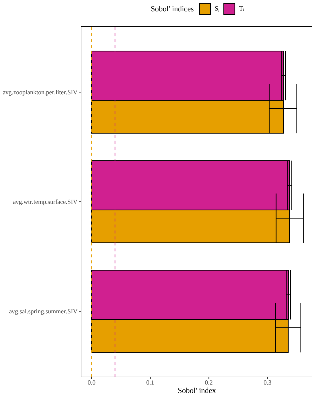
Figure 4. Results of a sensitivity analysis for the blueherringJuv model based on an arithmetic mean structure. Dashed lines represent baseline numerical approximation error for S_i and T_i ( i.e. , dummy variables).
