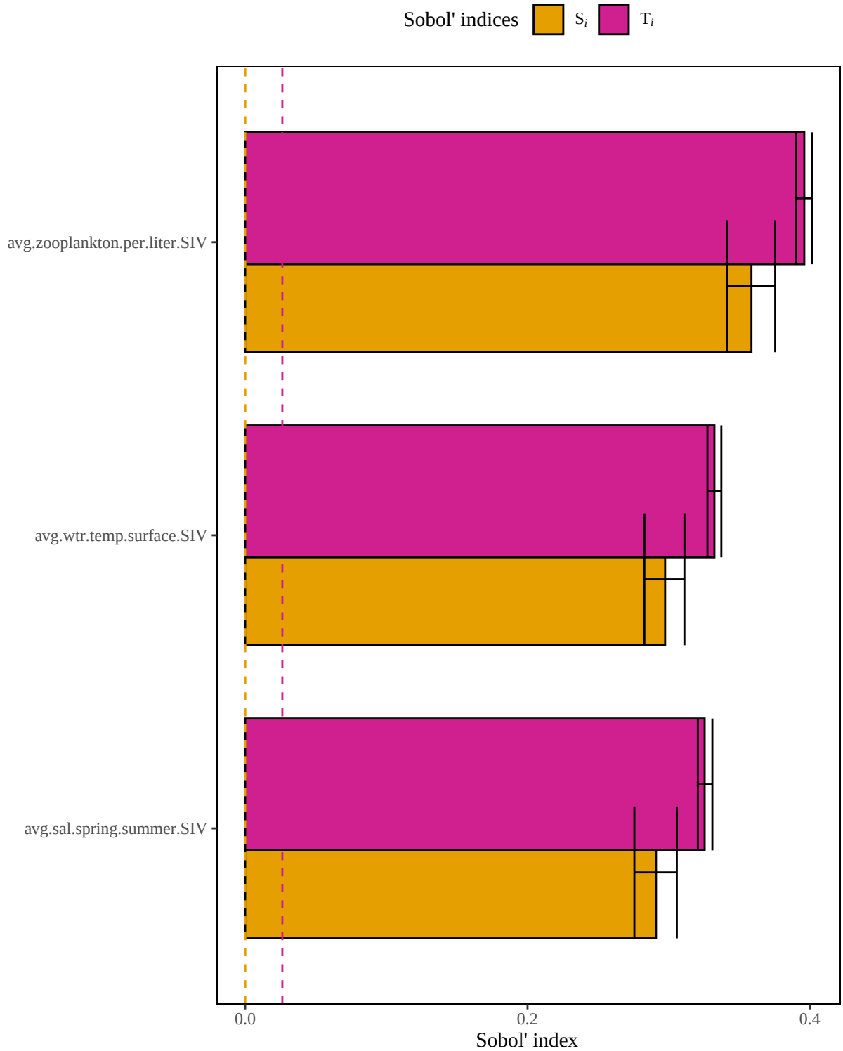
Figure 5. Results of a sensitivity analysis for the blueherringJuv model based on a geometric mean structure. Dashed lines represent baseline numerical approximation error for S_i and T_i ( i.e. , dummy variables).
